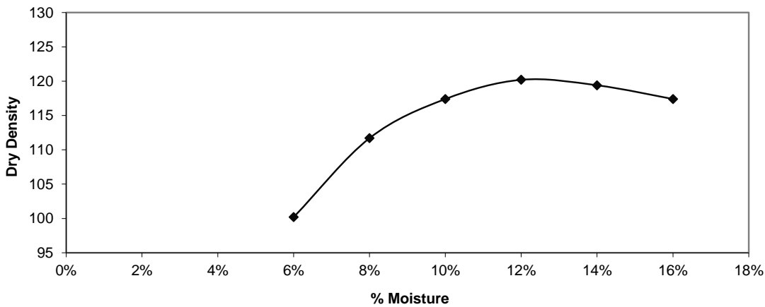
Moisture Density Relationship
